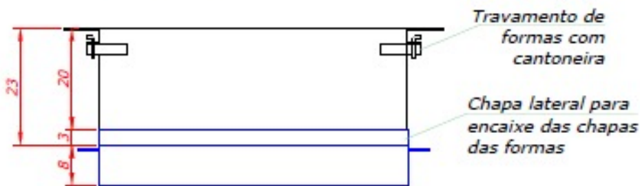
VISTA FRONTAL
